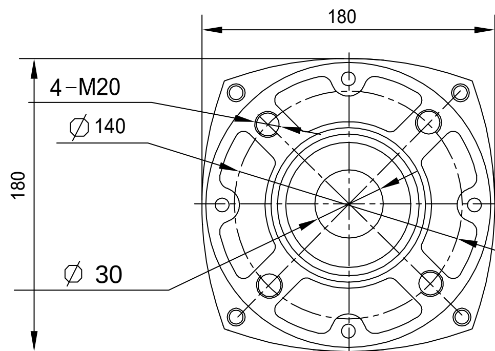
DETAIL K
