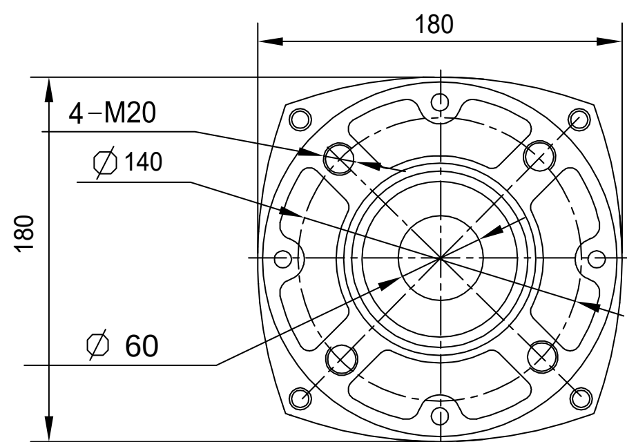
DETAIL K
