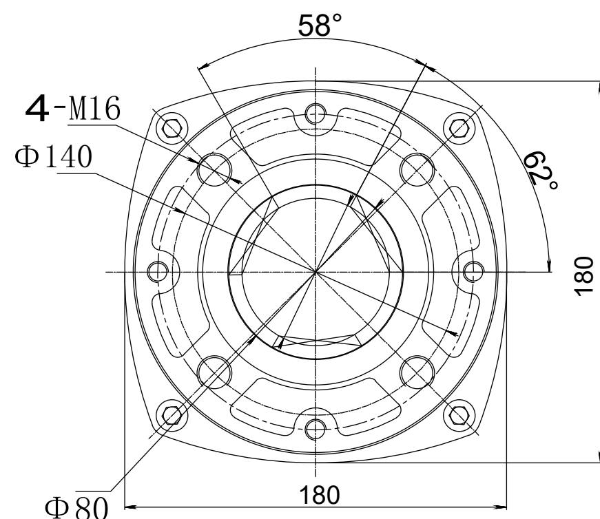
DETAIL K
