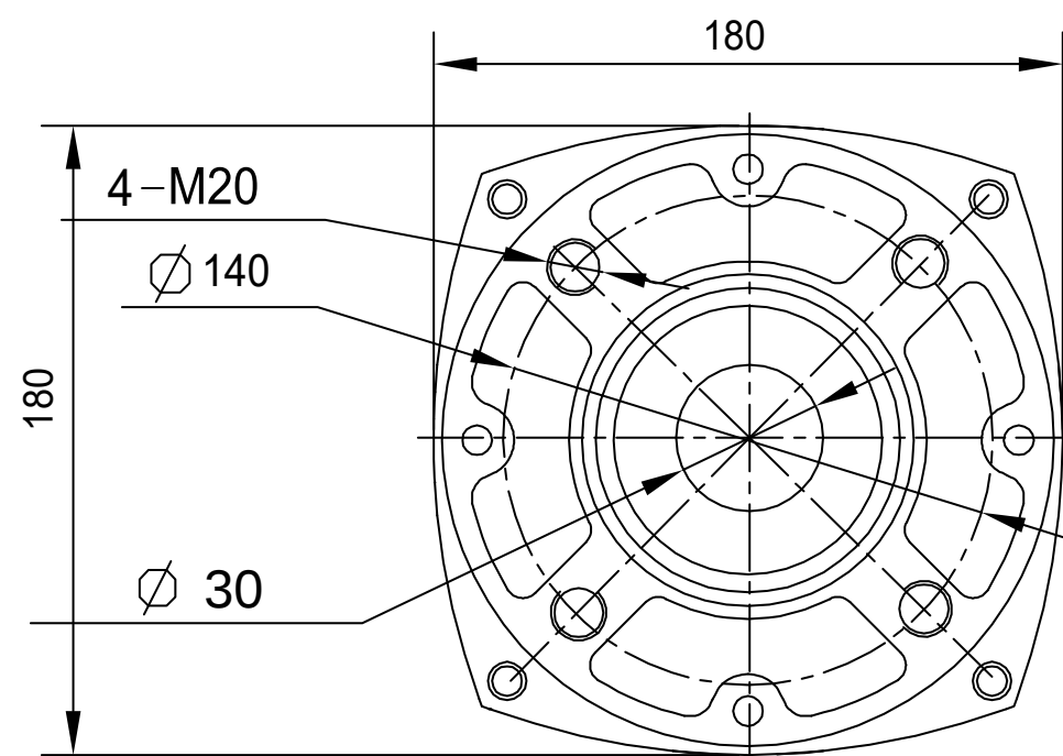
DETAIL K
