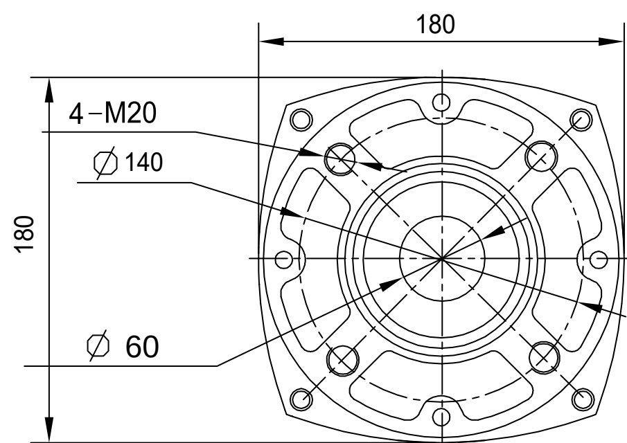
DETAIL K
