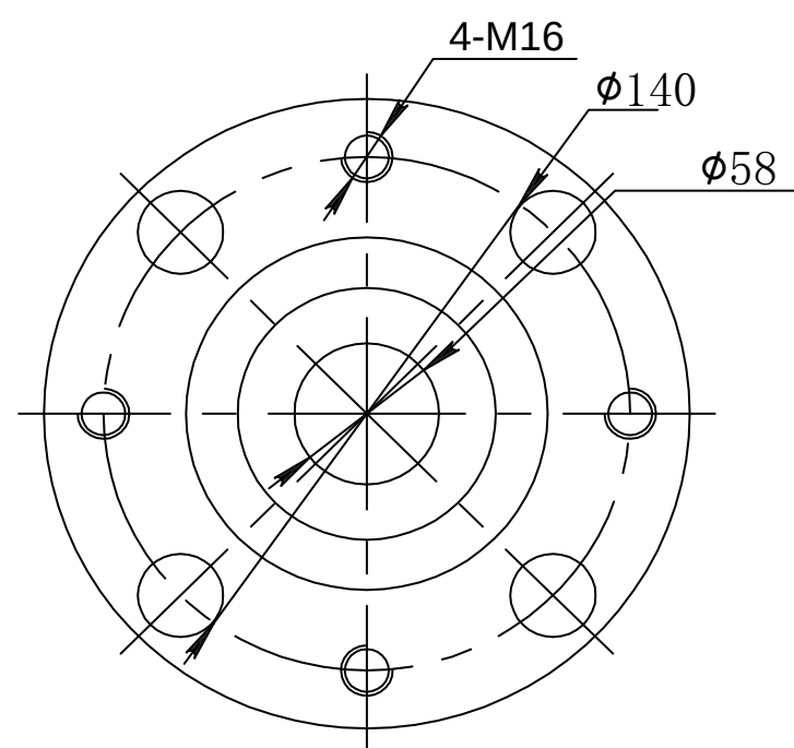
DETAIL K
