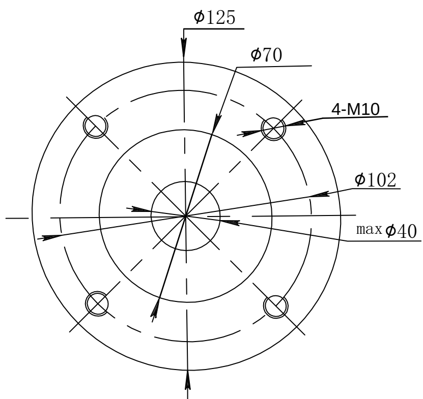
DETAIL K
