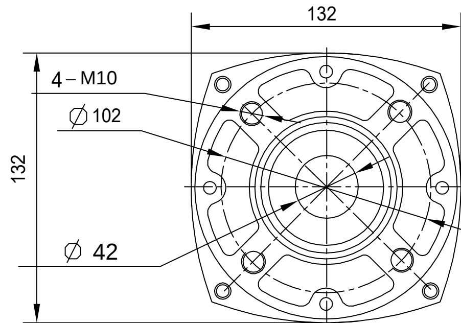
DETAIL K
