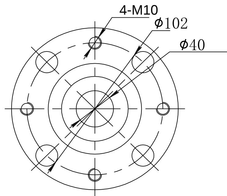
DETAIL K
