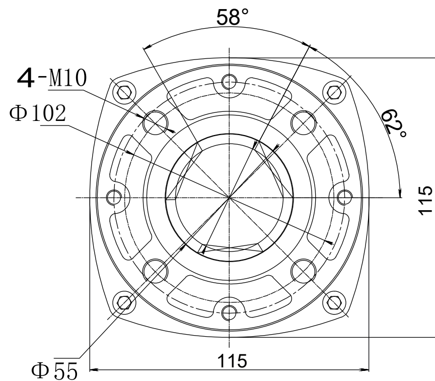
DETAIL K
